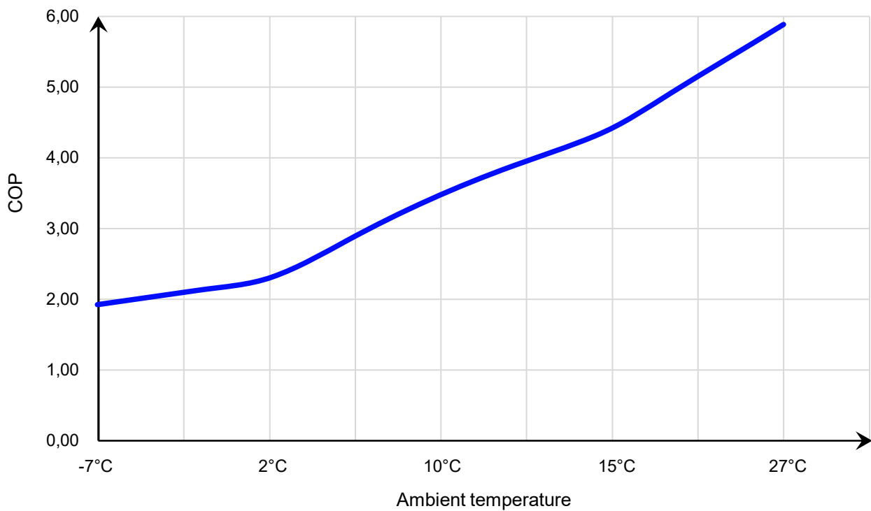
34-180620 COP Curve
