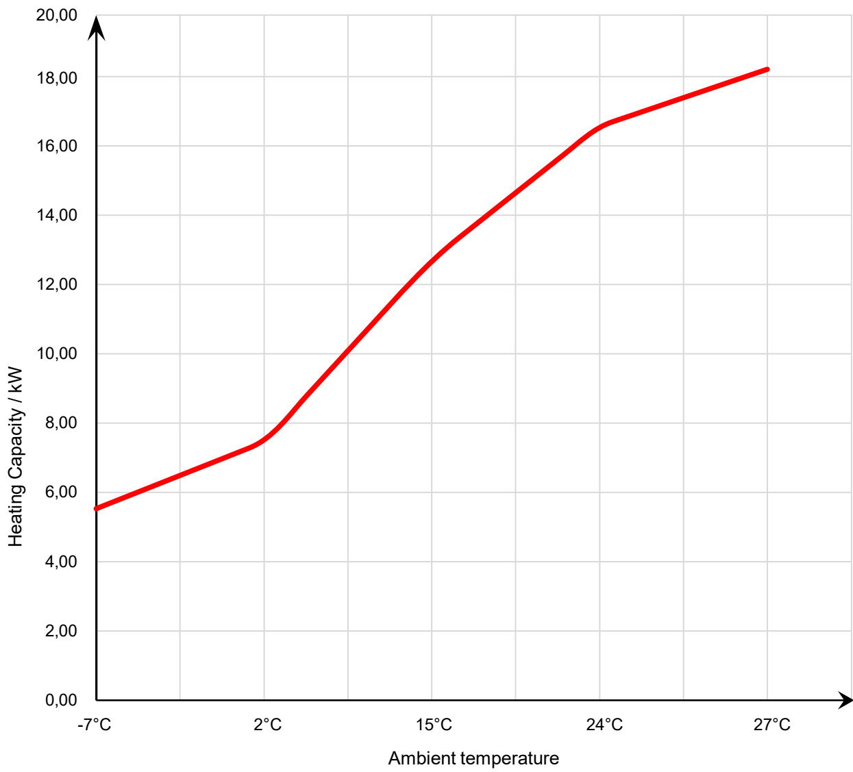
34-180626 Heating Capacity Curve
