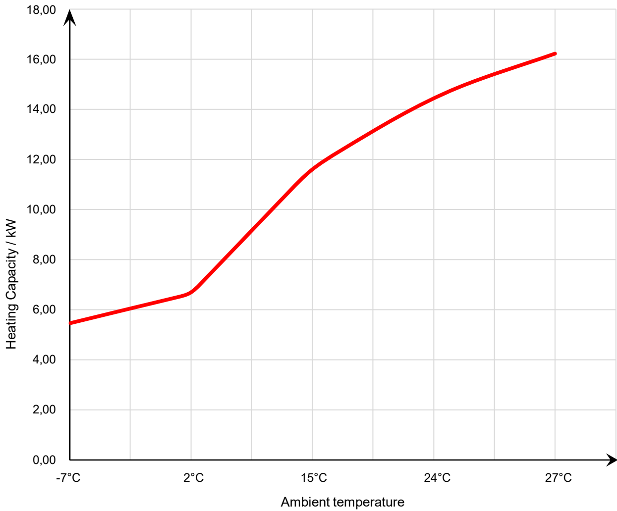
34-180624 Heating Capacity Curve
