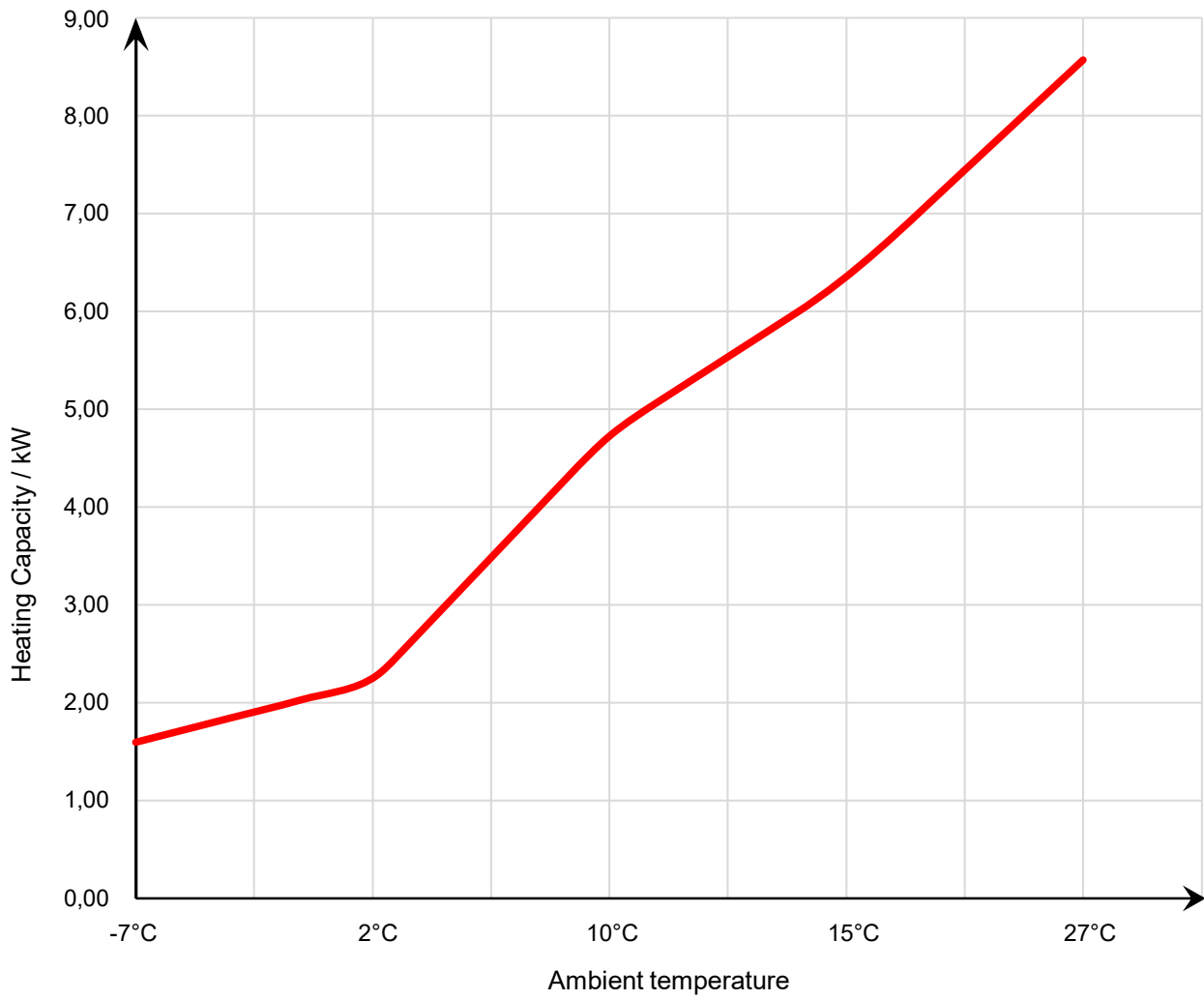
34-180620 Heating Capacity Curve
