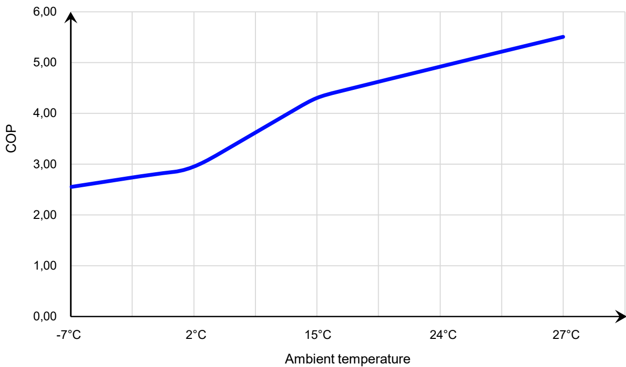
34-180624 COP Curve
