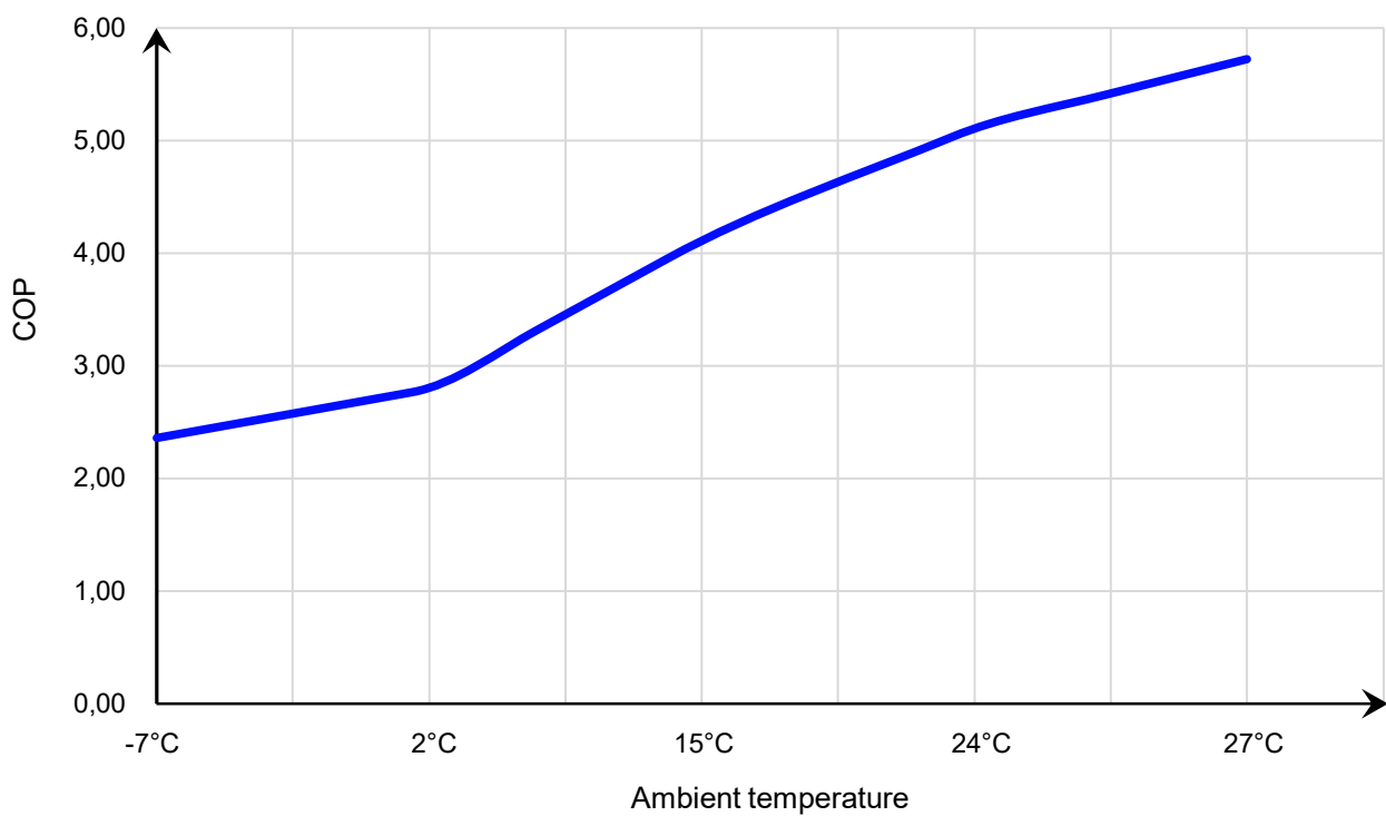
34-180626 COP Curve
